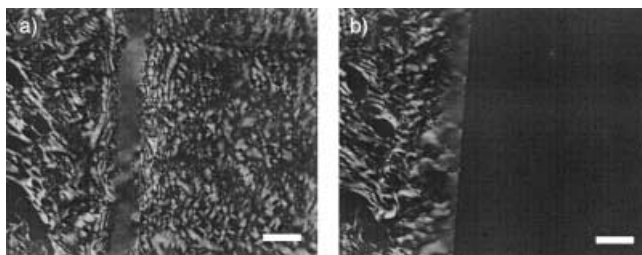
Figure 1. Microscopic images of the same section of a solution of 1 (20 wt %) in dodecane contained within a 4 μm thick electrooptic cell sandwiched between crossed polarizers: a) in the absence of an applied electric field; b) with an applied electric field of 9 V μm -1 . The electrode covers only the right side of the field of view. The length of the scale bar is 100 μm.
