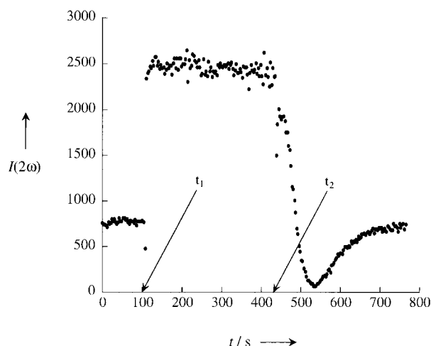
Figure 2. Plot of the second-harmonic signal intensity from 1 ( I(2\omega) ), in arbitrary units) versus time t . At time t_1 a field of 10 V μm -1 was applied, and at time t_2 the field was switched off.
